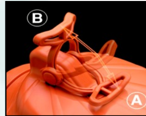
Manual closure lever to prevent flow in both directions.
